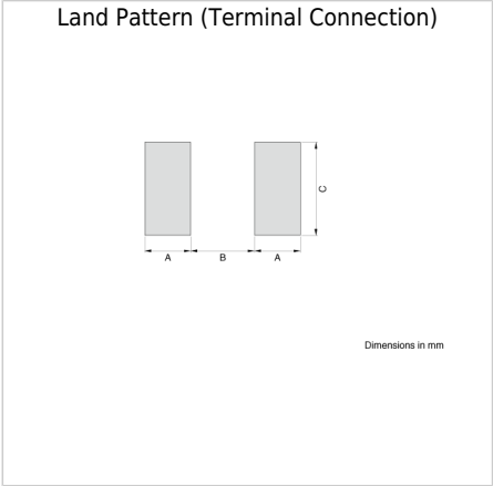
Land Pattern (Terminal Connection)
