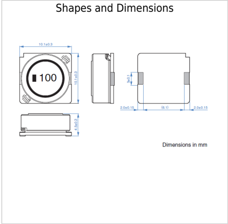
Shapes and Dimensions
