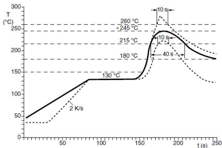
Figure 9 Soldering Reflow with Sn Solder
