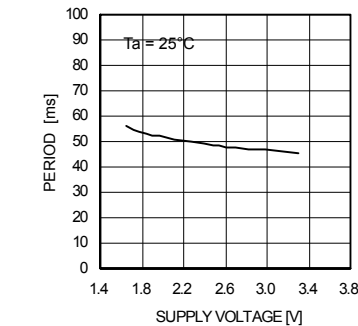
Fig.33 T P – Supply voltage
