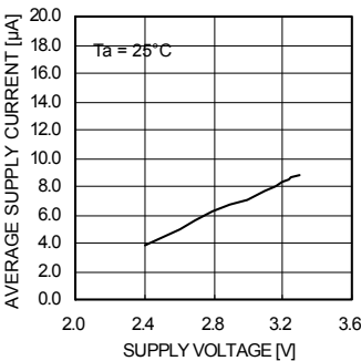
Fig. 17 I DD – Supply voltage
