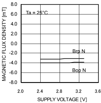
Fig. 13 Bop,Brp – Supply voltage
