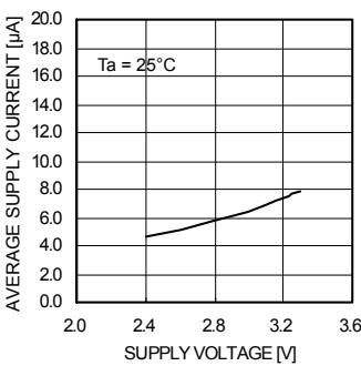
Fig. 11 I DD – Supply voltage
