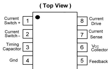
MSOP-8
