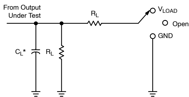
Figure 9. Load Circuit
