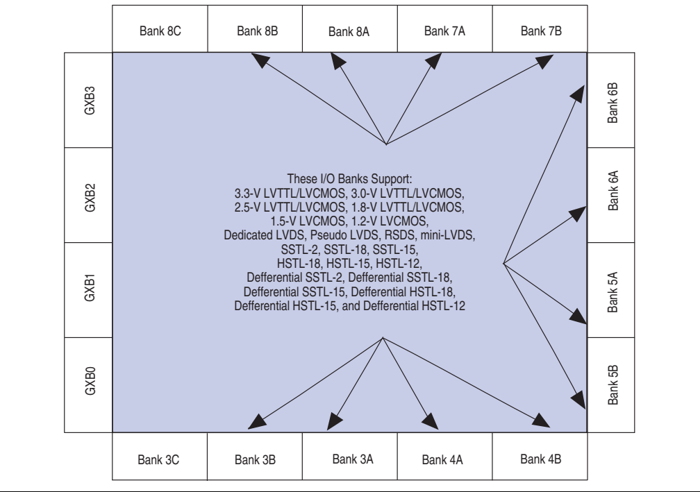
Figure 2-2. EP2AGX125 and EP2AGX260 Device I/O Bank Diagram
