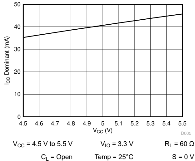
Figure 9-5. I_{CC} Dominant Current over V_{CC} Supply Voltage
