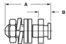
Part No. 206514-1
