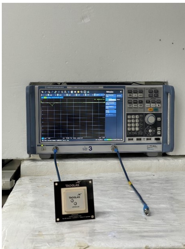
AA.215.201111 VNA Test Set-up
