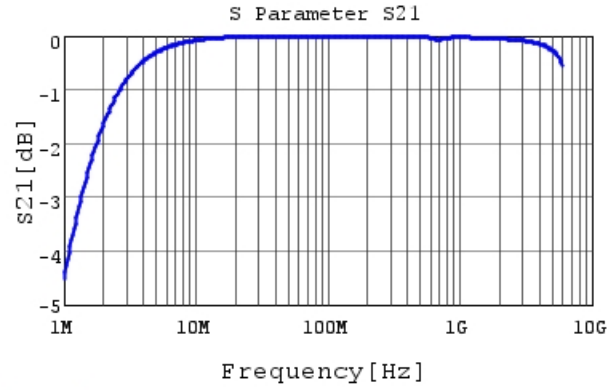
GCM1885C1H122JA16 S21 DCOV, 25degC
