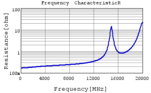
GJM1555C1H2R2BB01 R DCOV, 25degC
