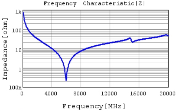
GJM1555C1H2R2BB01 |Z| DCOV, 25degC
