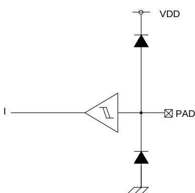
Figure 4. I/O Equivalent Circuit
