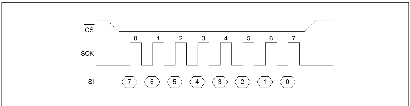
Figure 6 SPI mode 0
