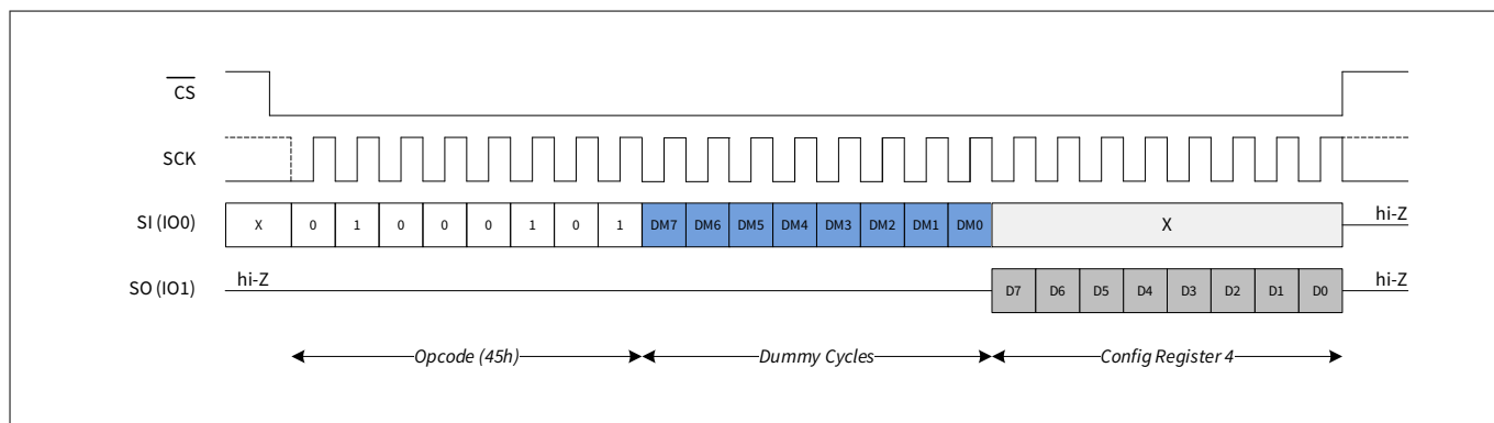
Figure 29 Read CR4 (RDCR4) in SPI mode
