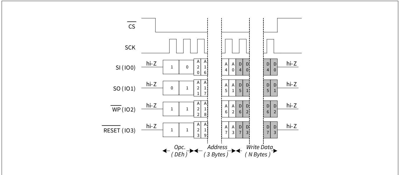
Figure 44 DDR write (DDRWRITE) in QPI mode
