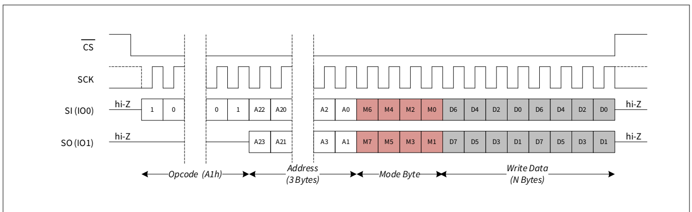
Figure 50 Dual I/O write (DIOW)
