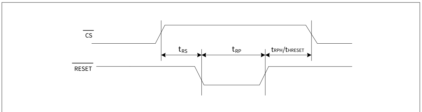
Figure 112 \overline{RESET} timing - SPI with QUAD clear (CR1[1]= '0') and QPI disabled (CR2[6] = '0')
