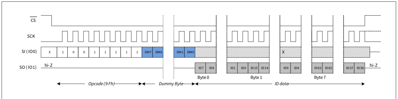
Figure 89 Read device ID (RDID) in SPI mode
