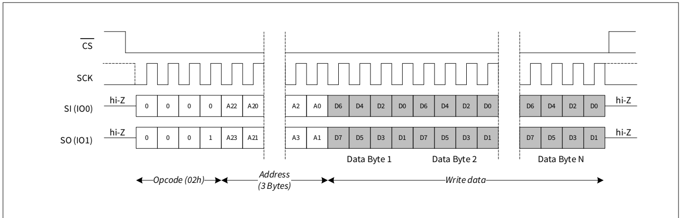
Figure 42 Memory write (WRITE) in DPI mode
