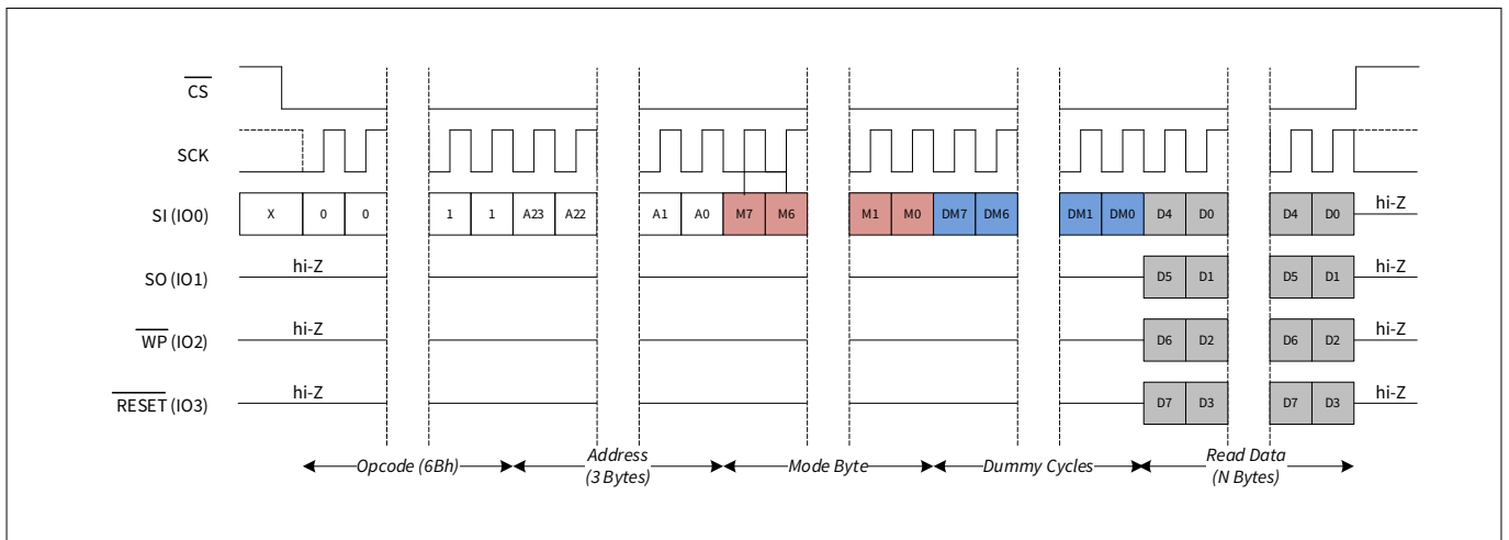
Figure 63 Quad output read (QOR)
