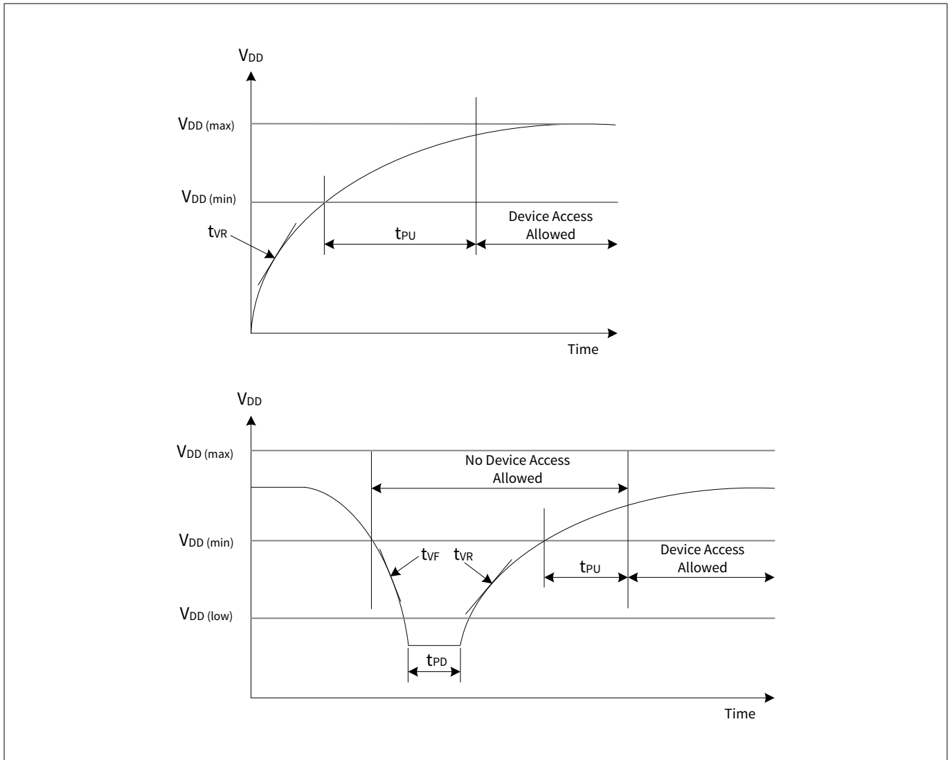
Figure 122 Power cycle timing
