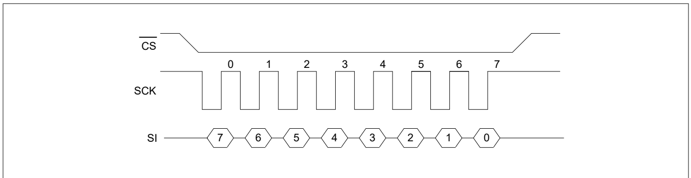
Figure 7 SPI mode 3
