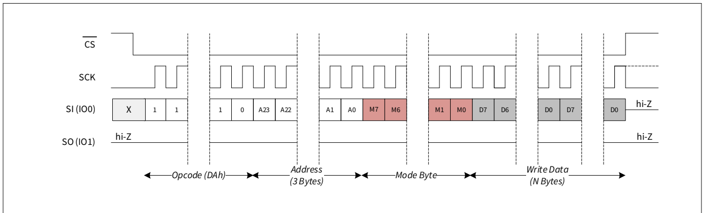
Figure 45 Fast write (FAST_WRITE) in SPI mode
