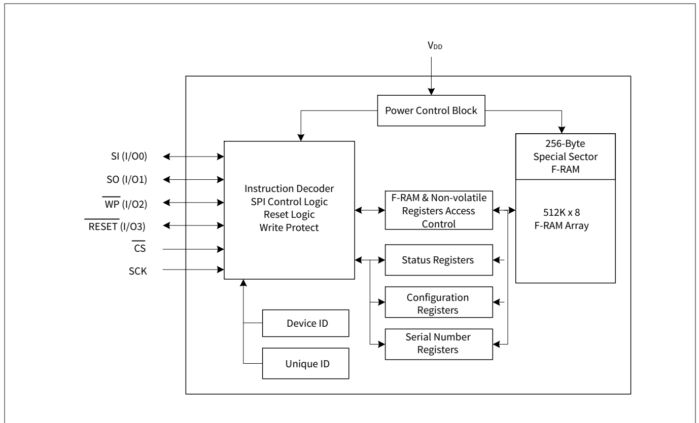
Figure 1 Block diagram
