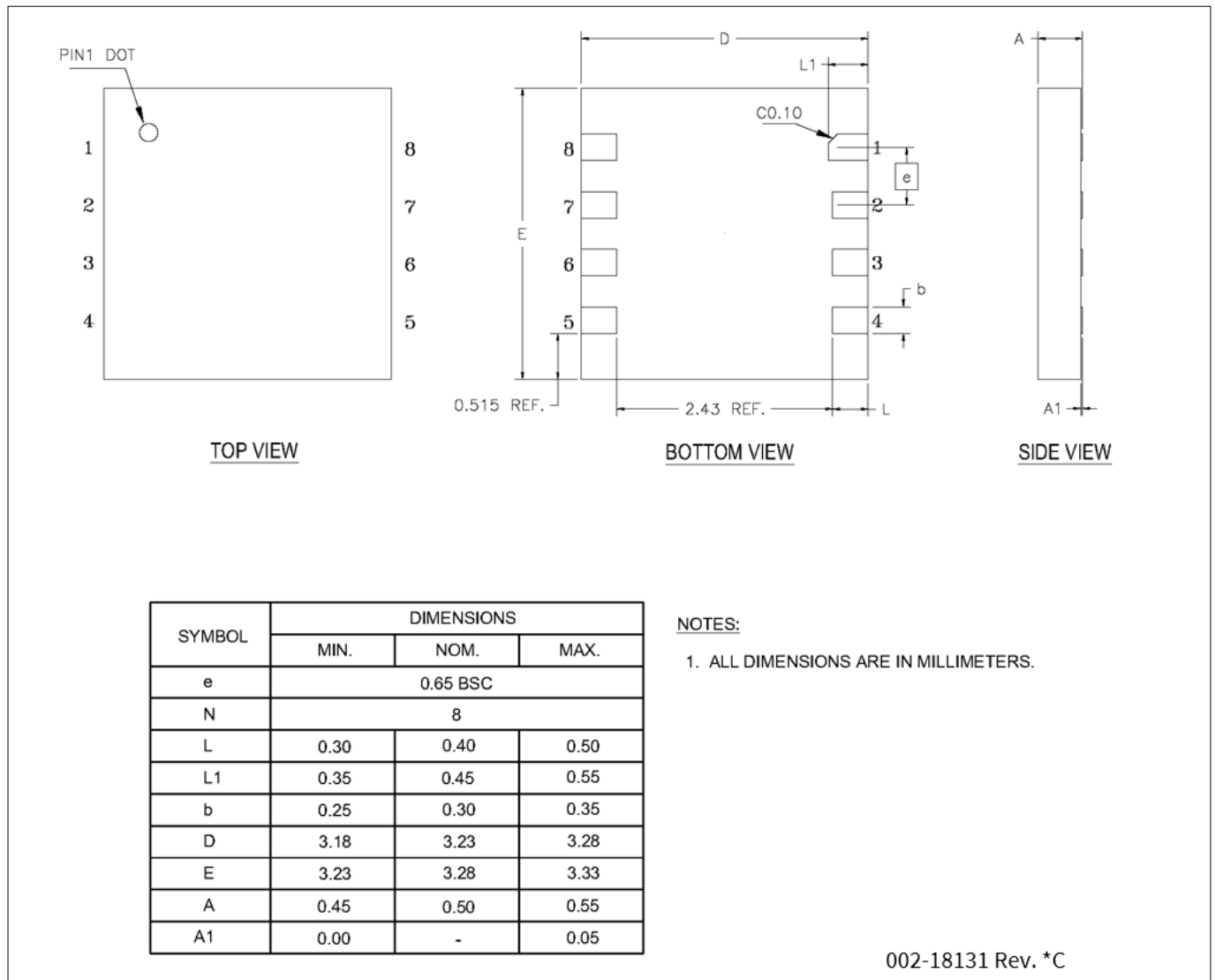
Figure 125 8-pin QFN (3.23 × 3.28 × 0.55 mm) LP08A package outline, (PG-VQFN-8), 002-18131
