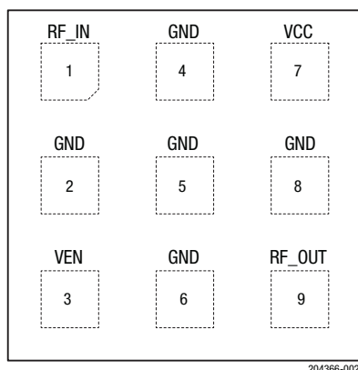
Figure 1. SKY65725-81 Pinout (Top View)
