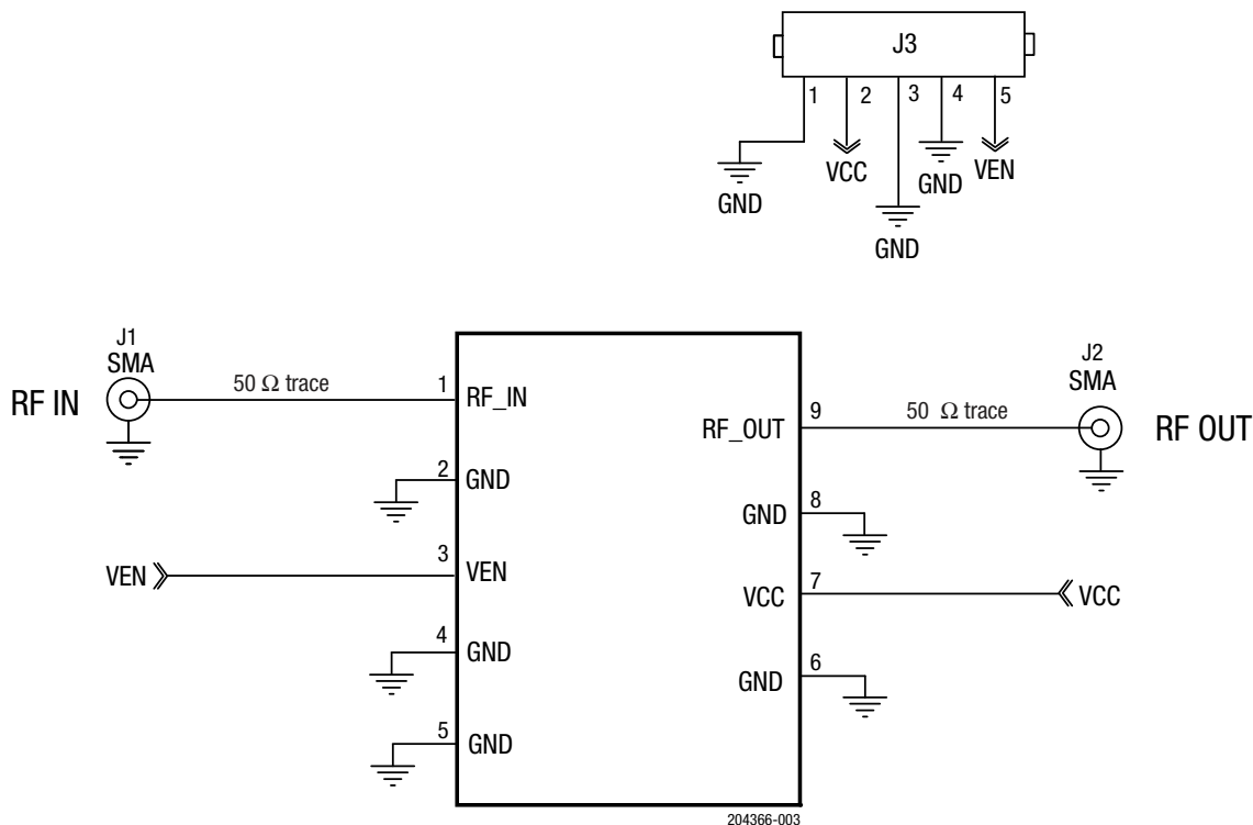
Figure 3. SKY65725-81 Evaluation Board Schematic
