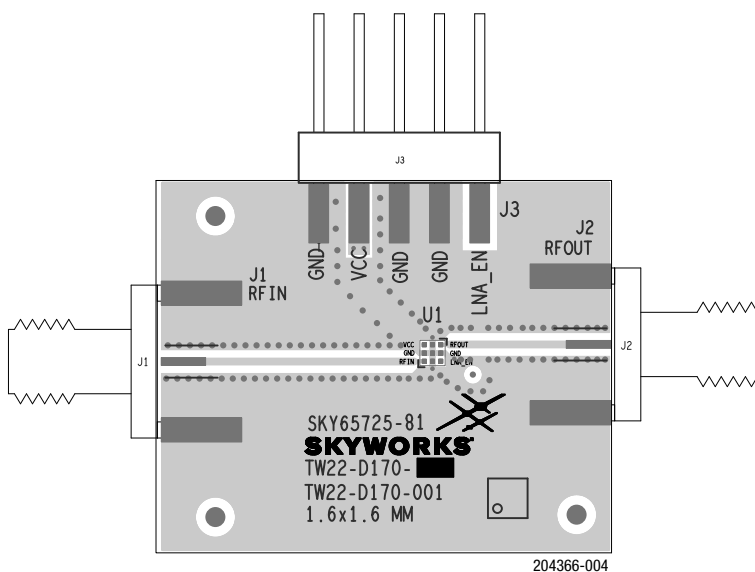
Figure 4. SKY65725-81 Evaluation Board Assembly Diagram
