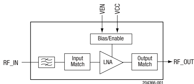
Figure 2. SKY65725-81 Block Diagram
