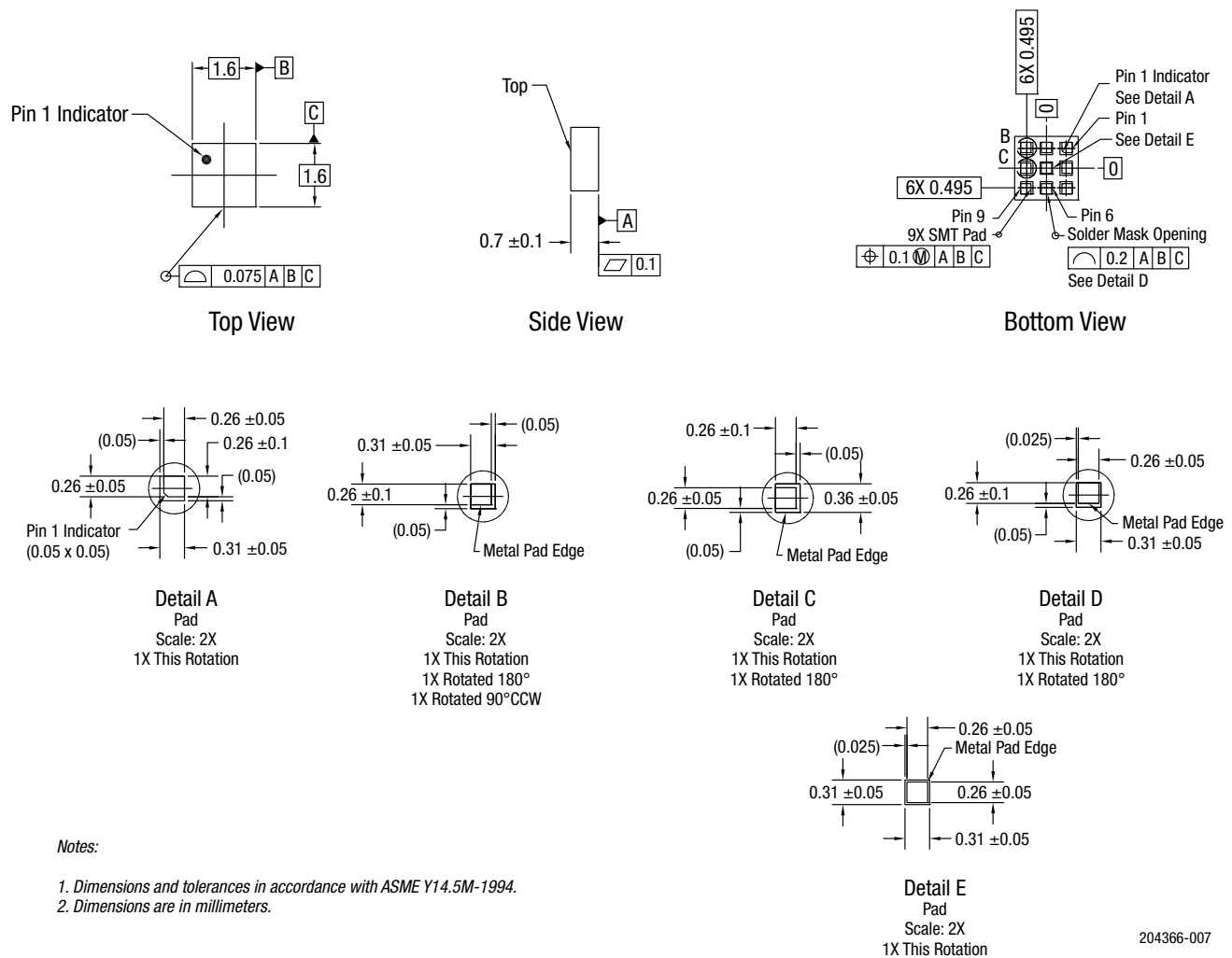
Figure 7. SKY65725-81 Package Dimensions
