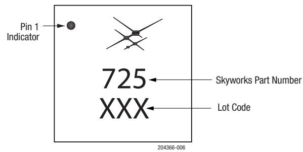
Figure 6. SKY65725-81 Typical Part Marking (Top View)
