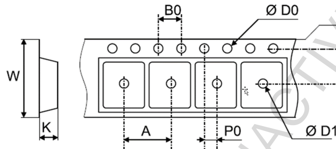
Figure 5. SOD128Flat carrier tape outline, bottom view (not in scale)
