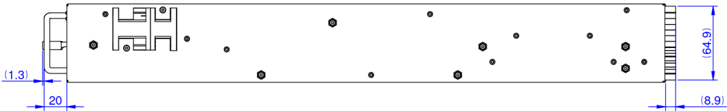
Figure 11. Bottom view
