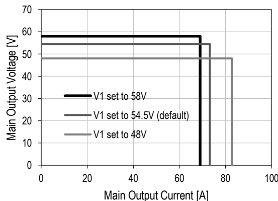
Figure 5. Output characteristics V_1
