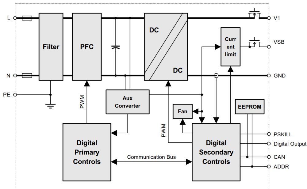
Figure 1. TET4000-48-069RAH Block Diagram
