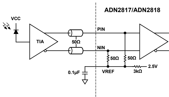
Figure 40. DC-Coupled Application
