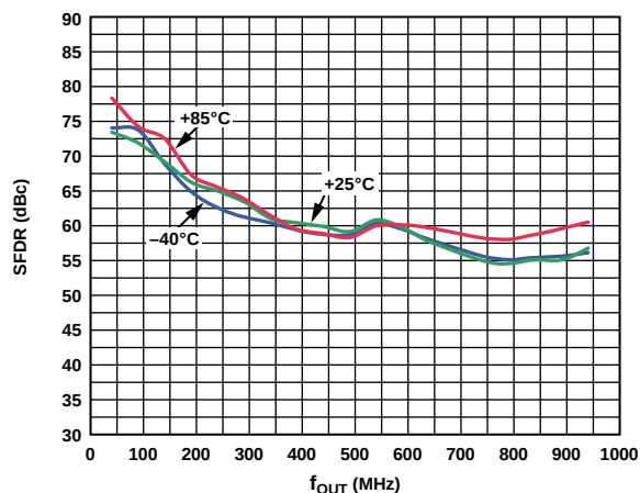
Figure 27. SFDR vs. f_{OUT} over Temperature
