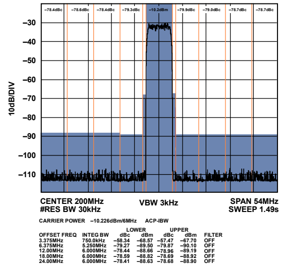
Figure 45. Low Band Narrow-Band ACLR
