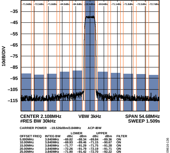
Figure 37. Typical Single-Carrier WCDMA ACLR Performance at 2.1 GHz, f_{DAC} = 2457.6 MSPS (Second Nyquist Zone)
