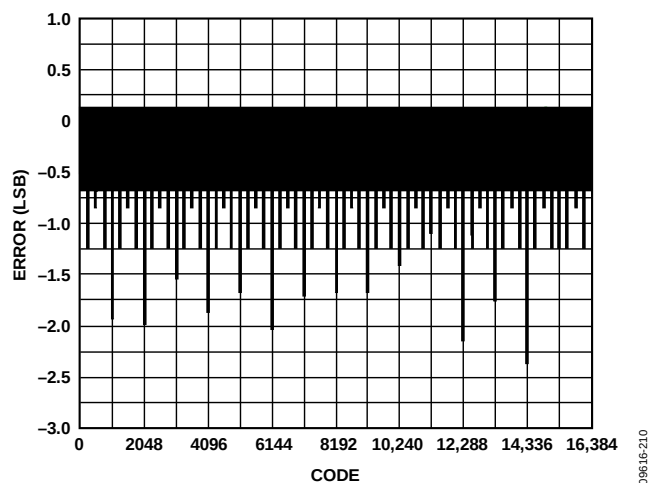
Figure 79. Typical DNL, 20 mA at 25°C
