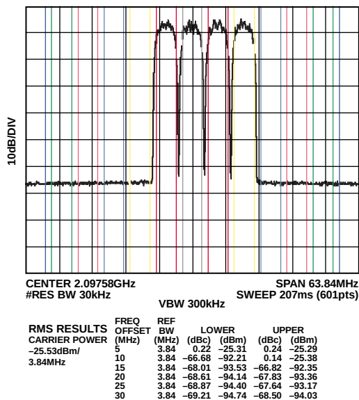
Figure 114. Typical Four-Carrier WCDMA ACLR Performance at 2.1 GHz, f_{DAC} = 2457.6 \text{ MSPS} (Second Nyquist Zone)
