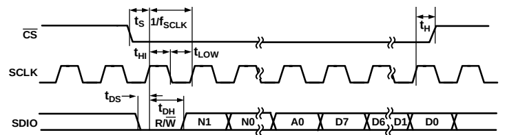
Figure 154. SPI Write Operation Timing
