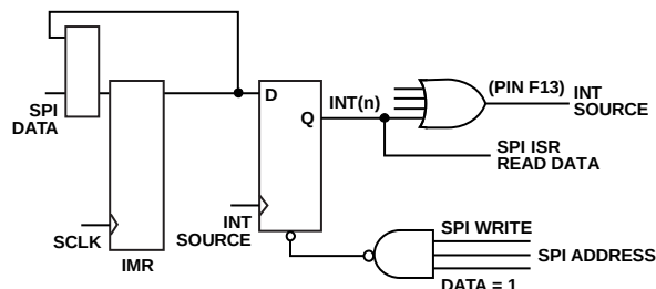
Figure 168. Interrupt Request Circuitry
