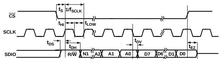
Figure 155. SPI 3-Wire Read Operation Timing
