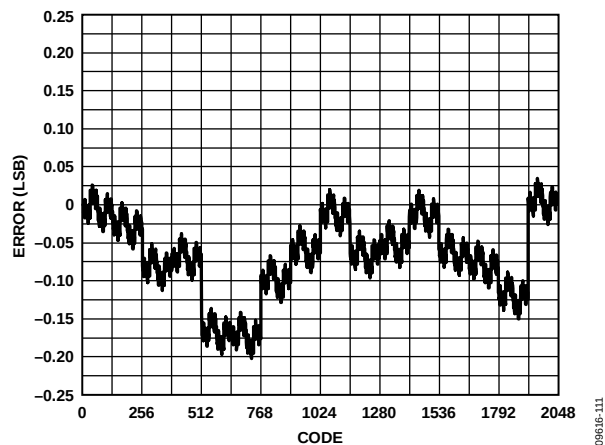
Figure 11. Typical INL, 10 mA at 25°C
