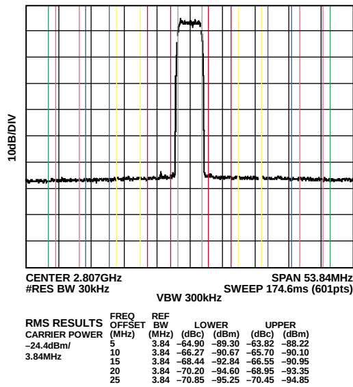
Figure 113. Typical Single-Carrier WCDMA ACLR Performance at 2.8 GHz, f_{DAC} = 2457.6 \text{ MSPS} (Third Nyquist Zone)
