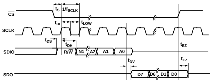
Figure 156. SPI 4-Wire Read Operation Timing
