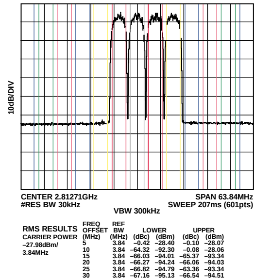
Figure 115. Typical Four-Carrier WCDMA ACLR Performance at 2.8 GHz, f_{DAC} = 2457.6 \text{ MSPS} (Third Nyquist Zone)
