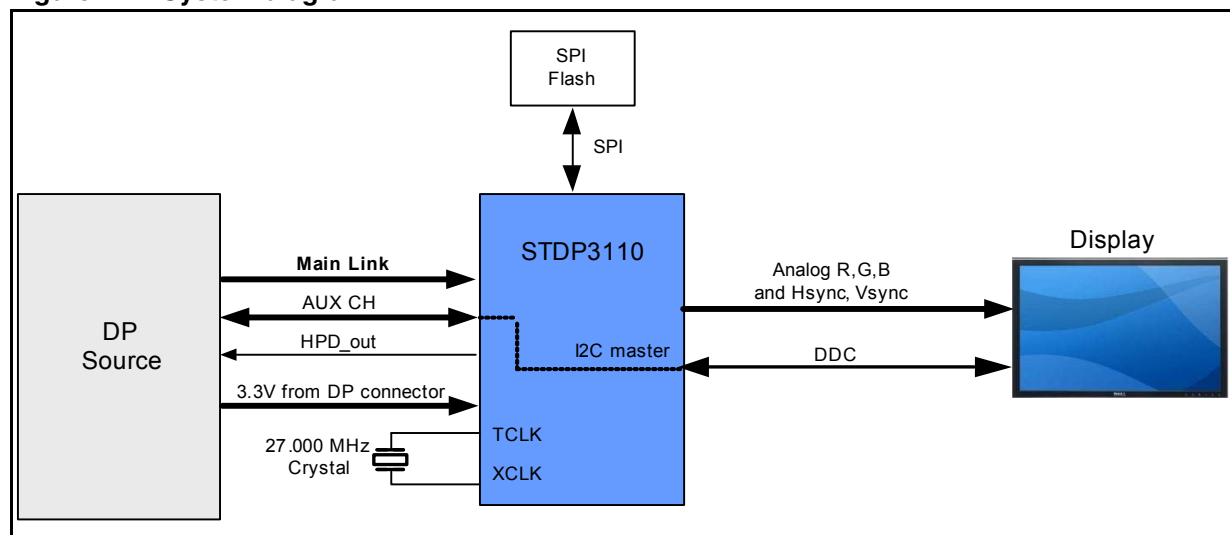
Figure 1. System diagram
