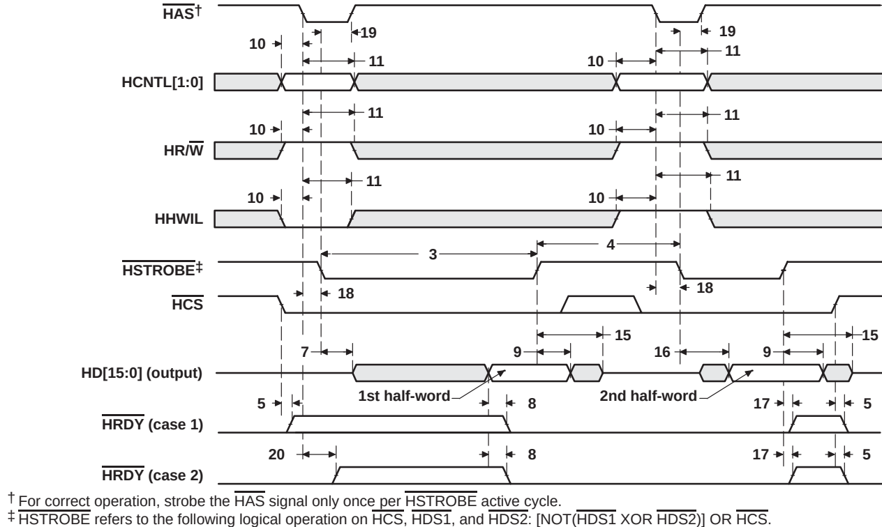
Figure 34. HPI Read Timing ( \overline{HAS} Used)
