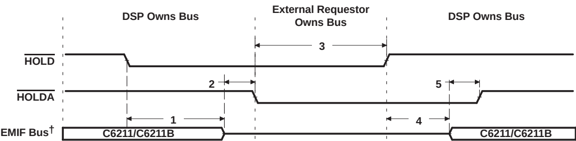
Figure 29. HOLD/HOLDA Timing
