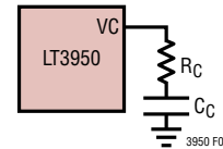
Figure 6. Typical Compensation
