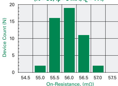
Typical On-Resistance Distribution (N = 50, I_F = 5 mA, I_L = 1 A)
