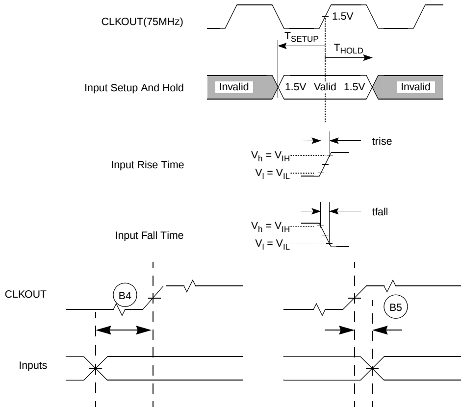
Figure 7. General Input Timing Requirements
