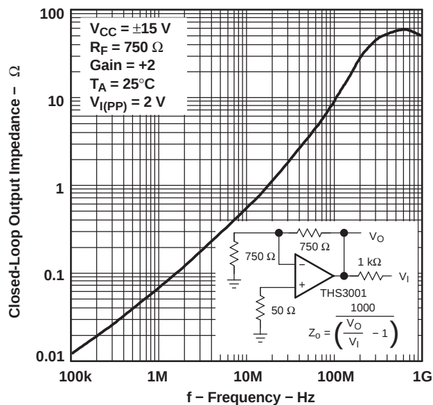
CLOSED-LOOP OUTPUT IMPEDANCE VS FREQUENCY
