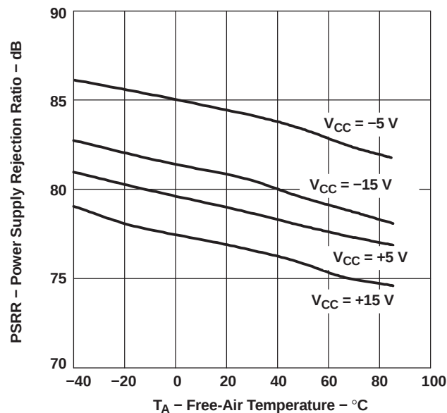
POWER SUPPLY REJECTION RATIO VS FREE-AIR TEMPERATURE
