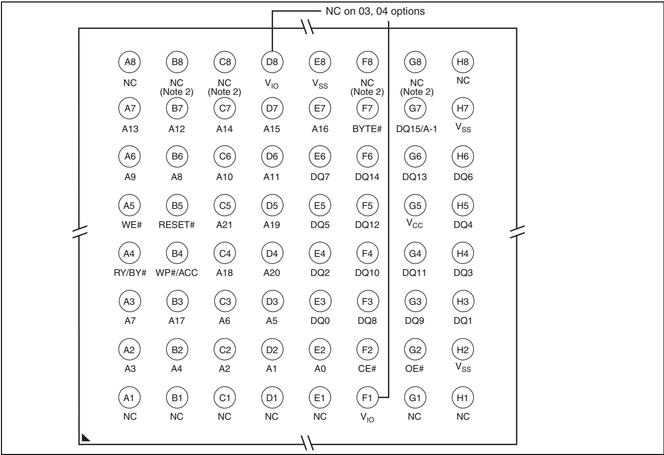
Figure 4 64-ball fortified BGA
