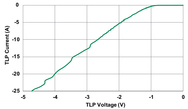
Negative Transmission Line Pulsing (TLP) Plot
