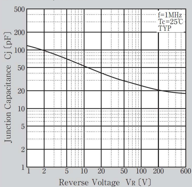
Junction Capacitance
