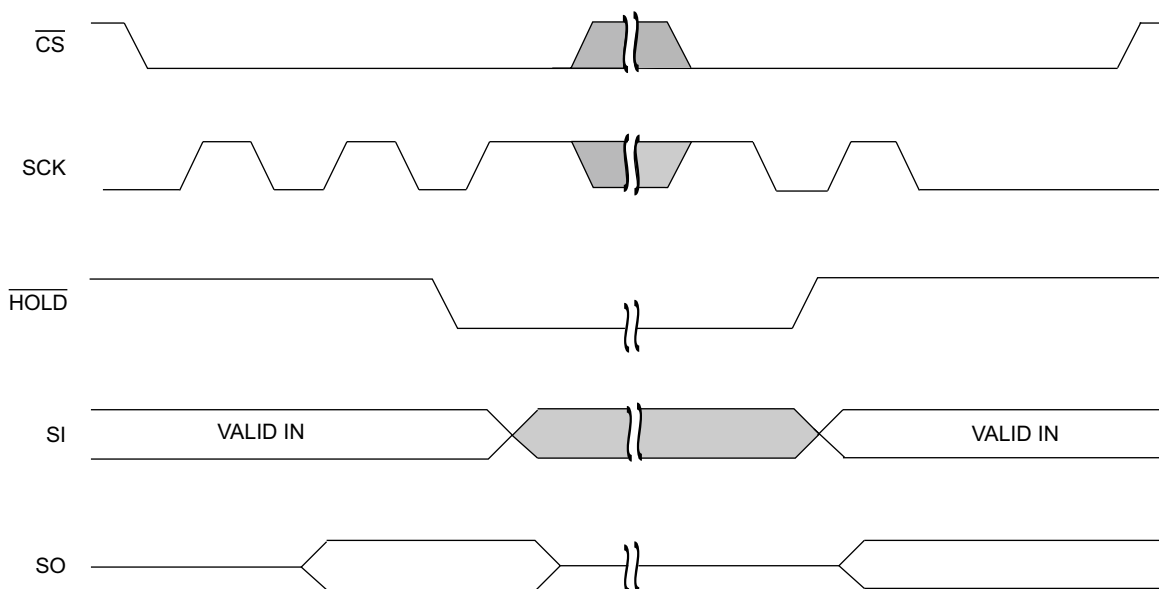
Figure 13. \overline{\text{HOLD}} Operation [2]
