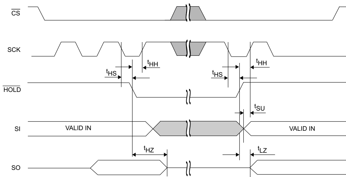
Figure 17. \overline{\text{HOLD}} Timing
