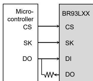
Figure 32-(b) Connection by 3 lines
