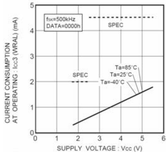
Figure 17. Consumption current at WRAL action ICC3 (WRAL, f_{SK}=500\text{kHz} )
