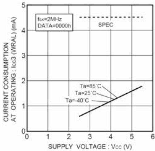
Figure 14. Consumption current at WRAL action ICC3 (WRAL, f_{SK}=2\text{MHz} )
