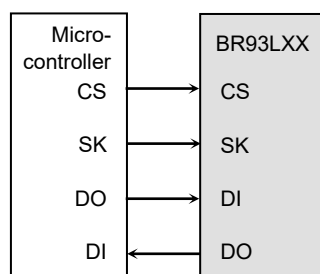
Figure 32-(a) Connection by 4 lines
