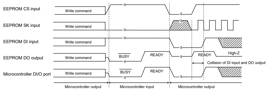
Figure 55. Collision timing at DI, DO direct connection
