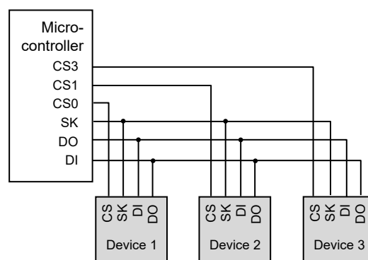
Figure 32-(c) Connection example of plural devices
