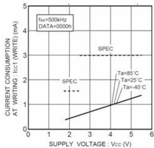
Figure 15. Current consumption at WRITE action ICC1 (WRITE, f_{SK}=500\text{kHz} )
