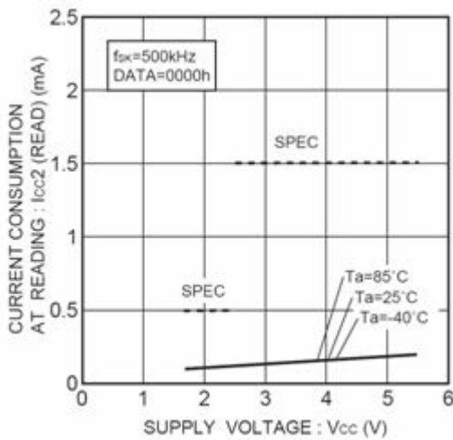
Figure 16. Consumption current at READ action ICC2 (READ, f_{SK}=500\text{kHz} )
