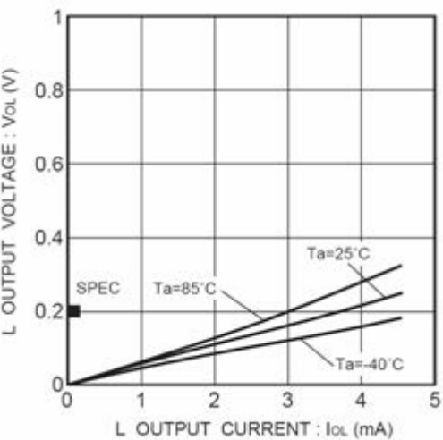
Figure 5. L output voltage V_{OL} - I_{OL} ( V_{CC}=2.5\text{V} )
