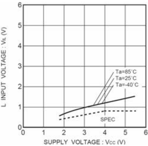
Figure 3. L input voltage V_{IL} (CS,SK,DI)
