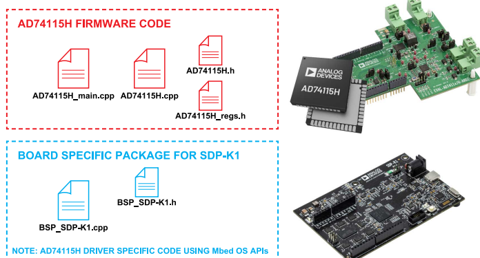
Figure 18. AD74115H No-OS Firmware Structure
