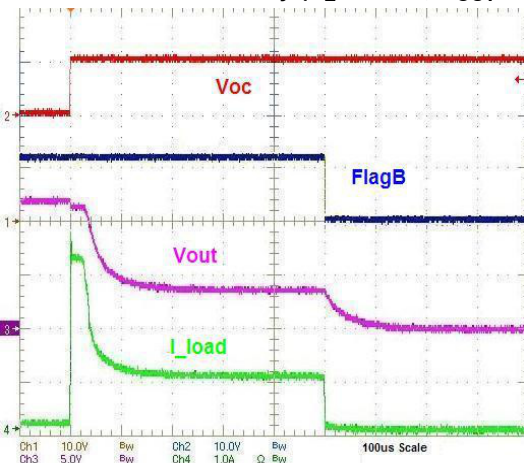
Figure 27. 12 V Blanking Time (Output Overloaded and t_{blank} Expired, FPF2700/01, I_{LIM} = 1\text{ A} , I_{LOAD} = 3.3\text{ A} , C_{OUT} = \mu\text{F} , R_{LOAD} = 500\ \Omega , V_{OC} (Note 2))
