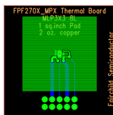
Figure 3. 80°C/W Mounted on a 1in 2 Pad of 2-oz. Copper
