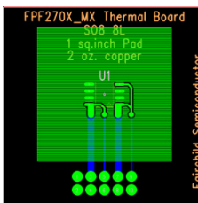
Figure 5. 102°C/W mounted on a 1in 2 Pad of 2-oz. Copper
