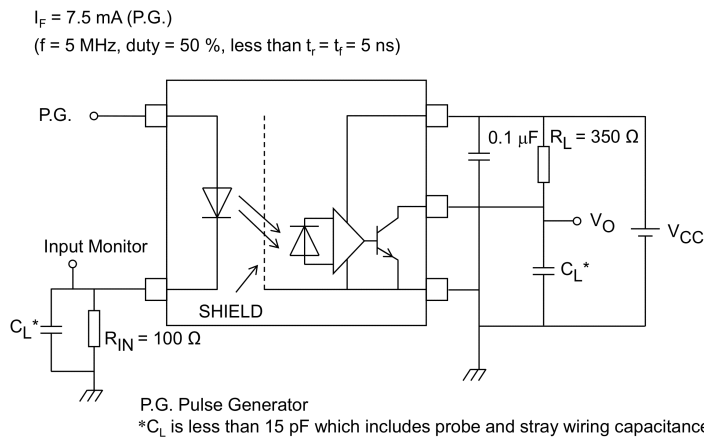
Fig. 12.1.5 Switching Time Test Circuit and Waveform
