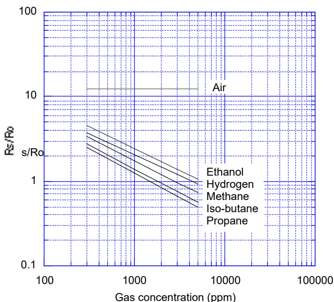
Sensitivity Characteristics:
