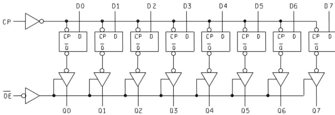
FIGURE 3. Logic diagram.
