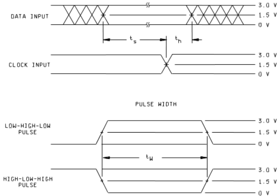
FIGURE 4. Switching waveforms and test circuit.
