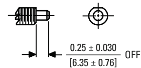
Push-to-Reset Actuation (Single and Two Pole)
