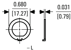
Locking Ring (Toggle)
