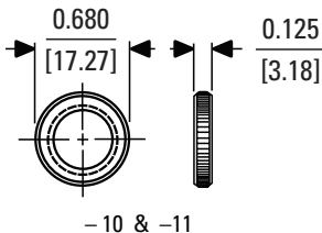
Knurled Nut
