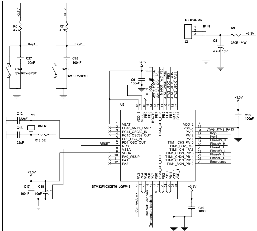
Figure 1. Microcontroller
