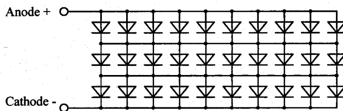
Equivalent circuit
