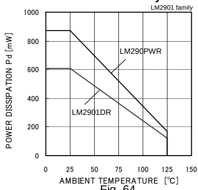
Fig. 64 Derating Curve
