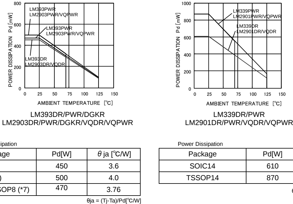
Fig.91 Derating Curves
