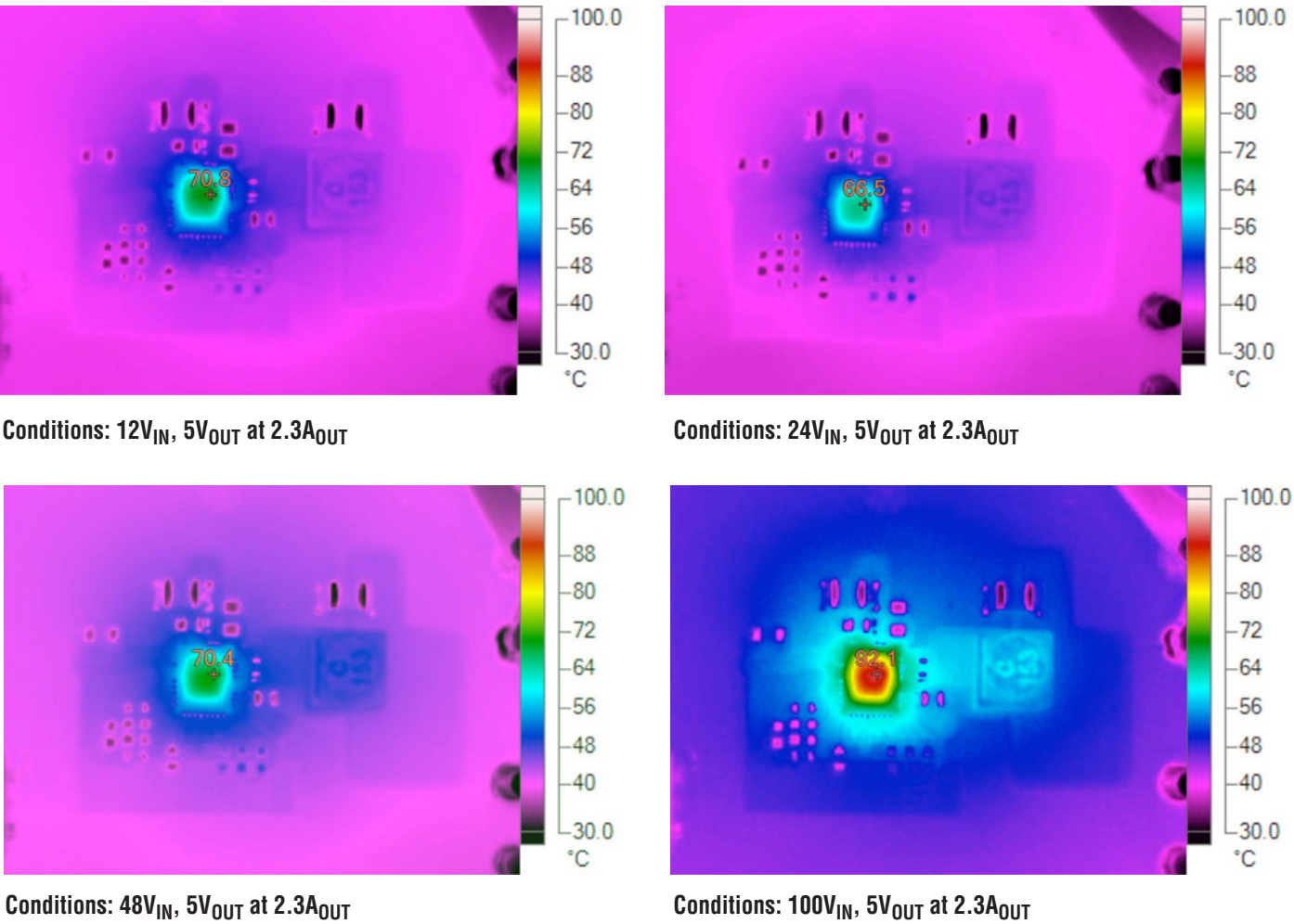
Figure 7. Thermal Plots (without Forced Air)
