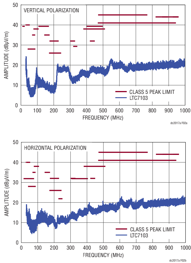
Figure 2. EMI Performance in CISPR 25 Radiated Emission Test ( 48V_{IN} from +VIN_EMI Turret Pin, 5V_{OUT}/2A , f_{SW} = 400kHz )
