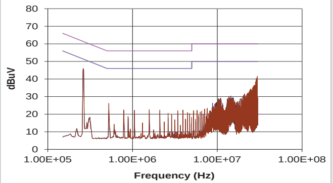
MTC1S2405MC
