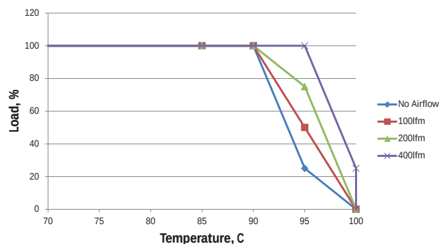
MTC1S2405MC - 18Vin
