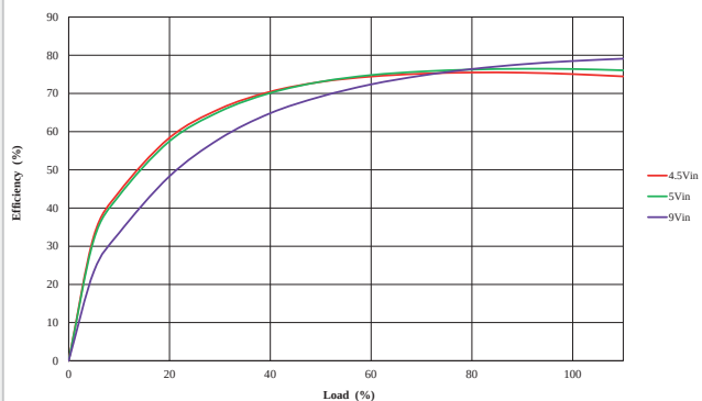
MTC1S1205MC
