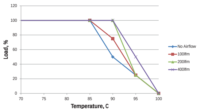
MTC1S2403MC - 18Vin
