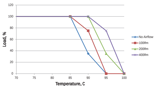
MTC1S2412MC - 18Vin
