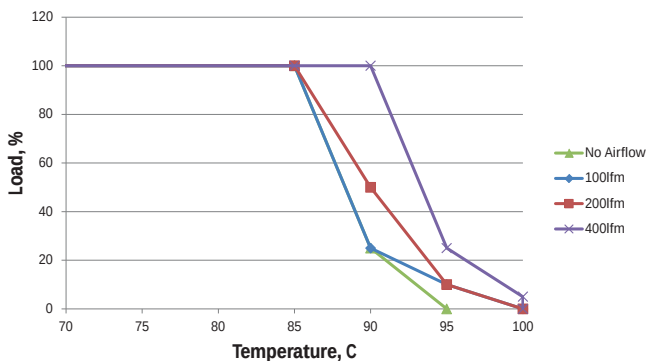
MTC1S1212MC - 18Vin
