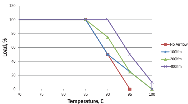
MTC1S1212MC- 12Vin
