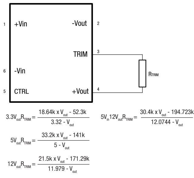
Figure 1. Trim connections to decrease the output voltage
