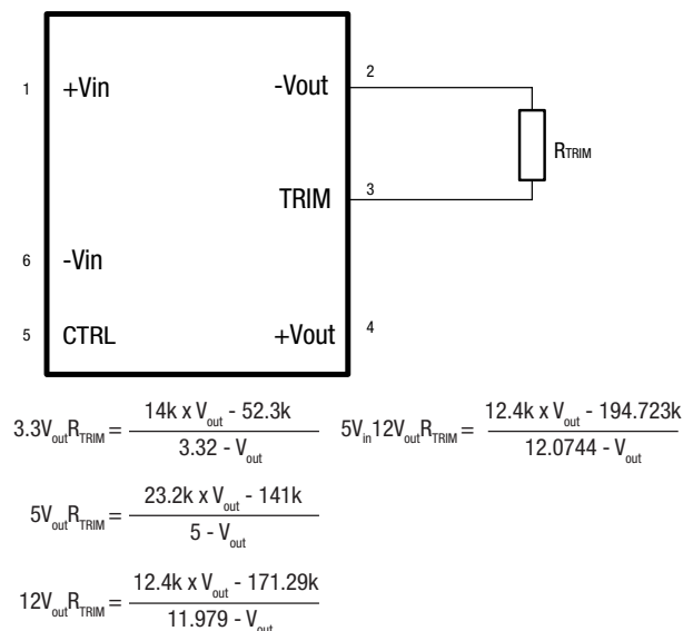
Figure 2. Trim connections to increase the output voltage
