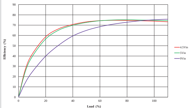
MTC1S0512MC
