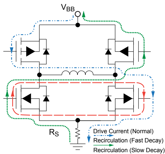
Figure 1 — Load-Current Paths
