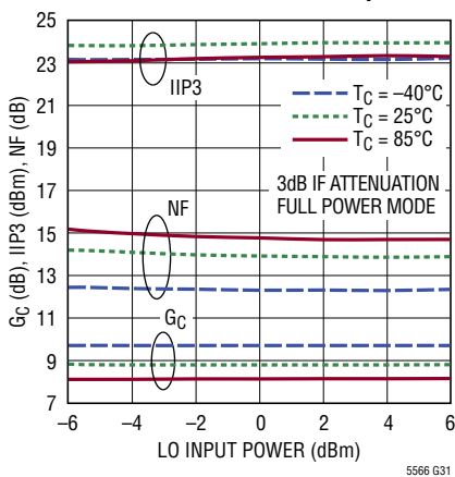
1.9GHz Conv Gain, IIP3 and SSB NF vs LO Power and Case Temperature
