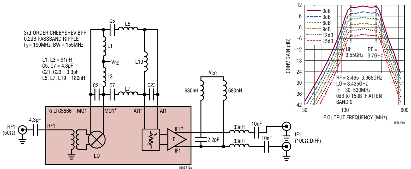
Figure 19. Test Circuit and Measured Conversion Gain with 3rd-Order Bandpass Interstage Filter
