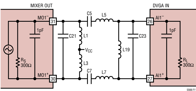
Figure 11. 3rd-Order Bandpass Filter Realization
