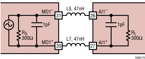
Figure 10. Equivalent Lowpass Filter Schematic
