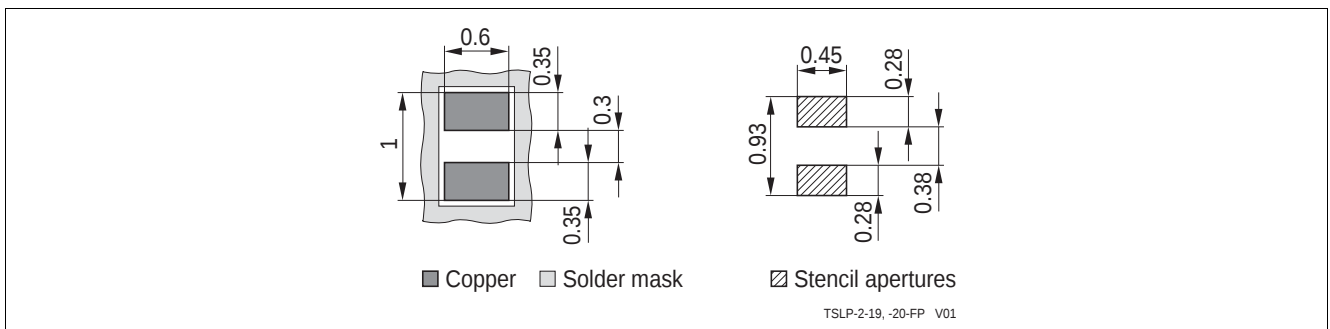
Figure 21 TSLP-2-20 Footprint
