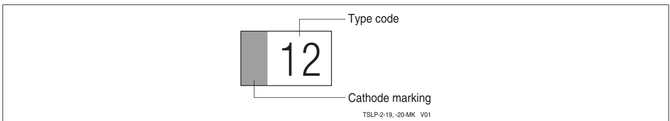
Figure 23 TSLP-2-20 Marking (example)
