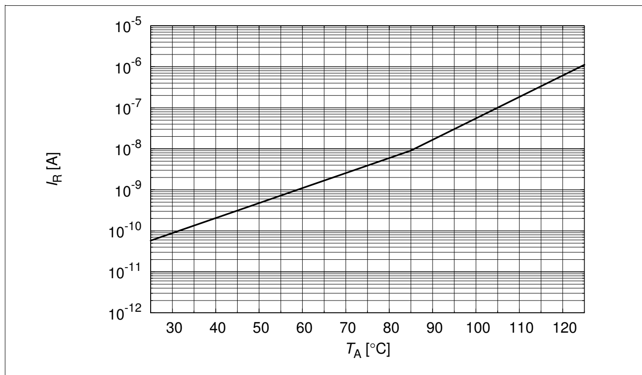
Figure 4 Reverse current: I_R = f(T_A) , V_R = 5.5\text{ V}
