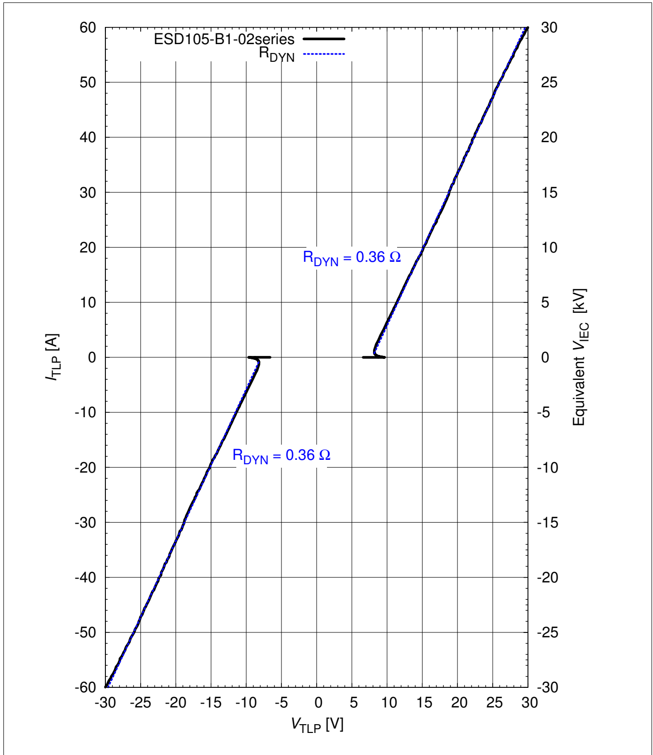
Figure 7 Clamping voltage (TLP): I_{TLP} = f(V_{TLP}) according ANSI/ESD STM5.5.1 - Electrostatic Discharge Sensitivity Testing using Transmission Line Pulse (TLP) Model. TLP conditions: Z_0 = 50\text{ }\Omega , t_p = 100\text{ ns} , t_r = 0.6\text{ ns} , I_{TLP} and V_{TLP} averaging window: t_1 = \text{ns} to t_2 = 60\text{ ns} , extraction of dynamic resistance using squares fit to TLP characteristics between I_{TLP1} = 10\text{ A} and I_{TLP2} = 50\text{ A} . Please refer to Application Note AN210[1]
