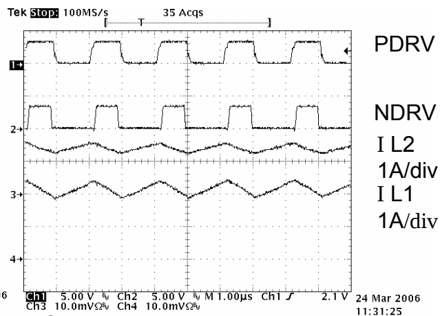
Switching Behavior, V_{IN}=3.3V
