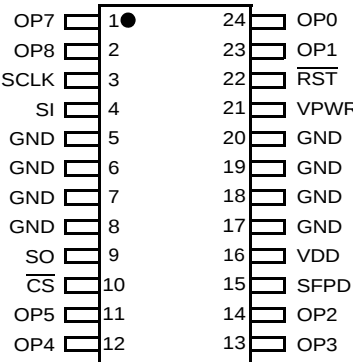
Figure 3. 33298 Pin Connections
