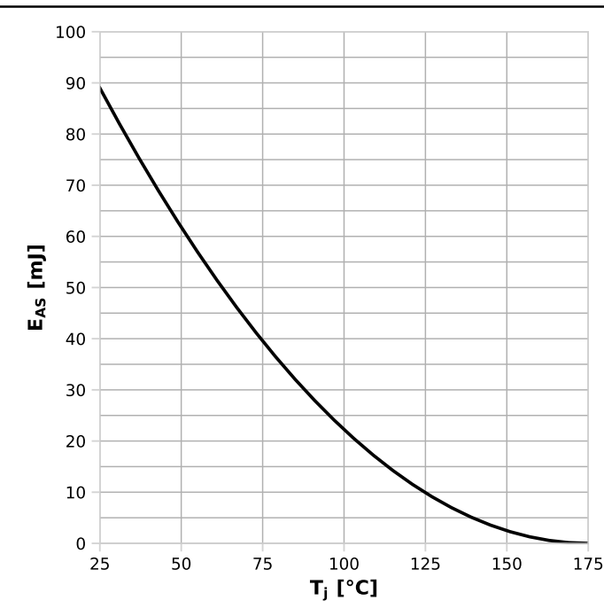
Diagram 13: Avalanche energy
