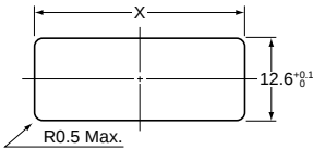
Diagram of recommended locations for panel mounting holes
