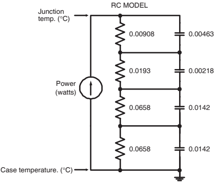
FIGURE 19b, TRANSIENT THERMAL IMPEDANCE MODEL
