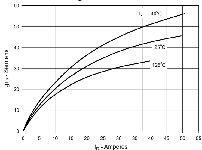
Fig. 8. Transconductance
