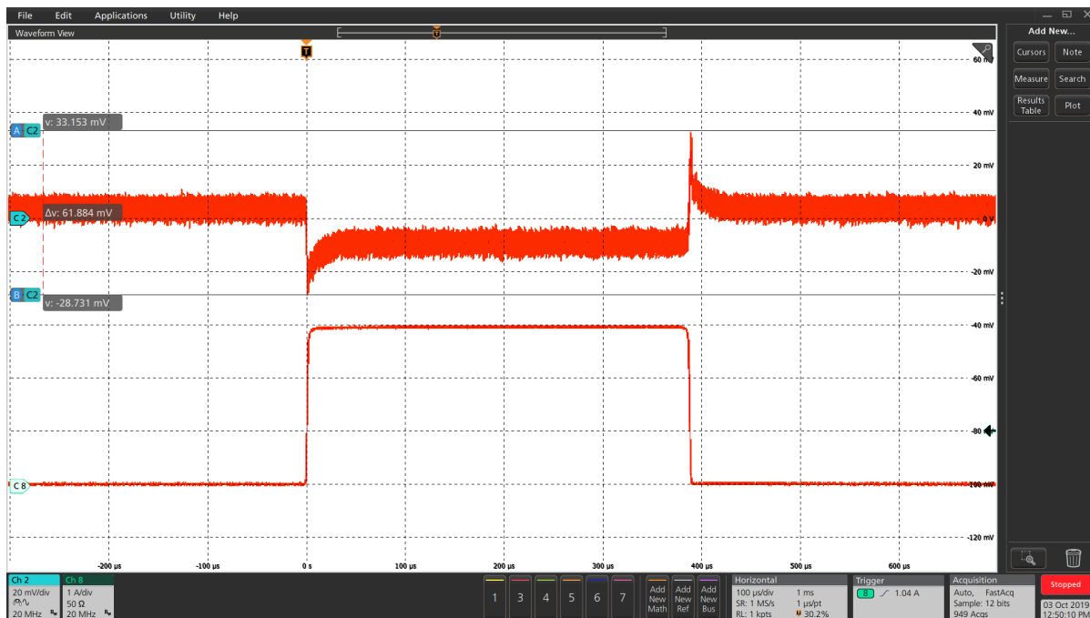
Figure 28 Transient response 0A to 3A (Ch6: I_{OUT} , Ch2: V_{OUT} ), peak-peak deviation=62mV
